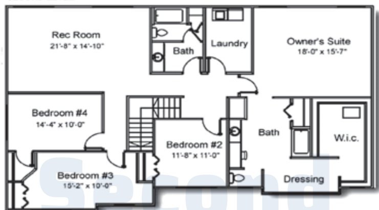
SECOND LEVEL
