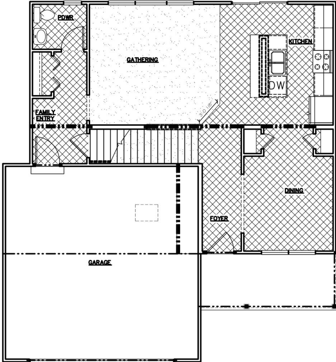
THE MAGNOLIA POPULAR DESIGN OPTIONS Main Floor
