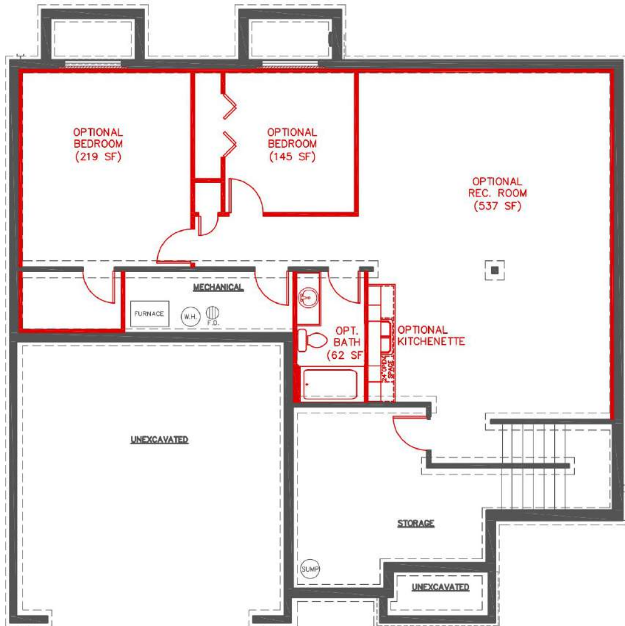
THE AUSTEN POPULAR DESIGN OPTIONS Lower Level
